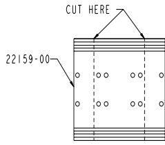
VIEW G (TO BE CUT ONLY WHEN USING WITH 22852-03)
